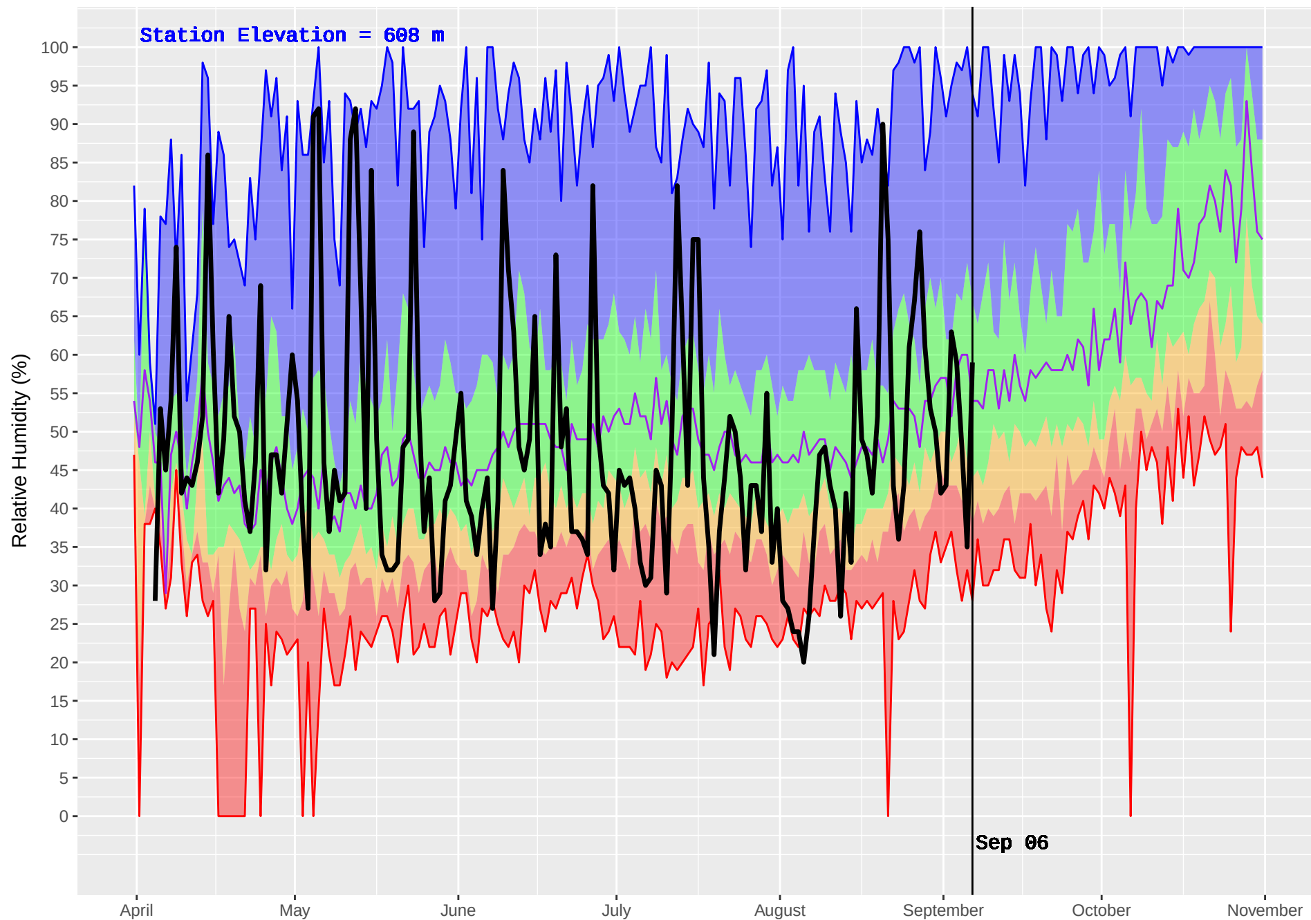
HOUSTON(DUNGATE) (162) : Historical (1974–2016) and Current (2017) Noon Relative Humidity
