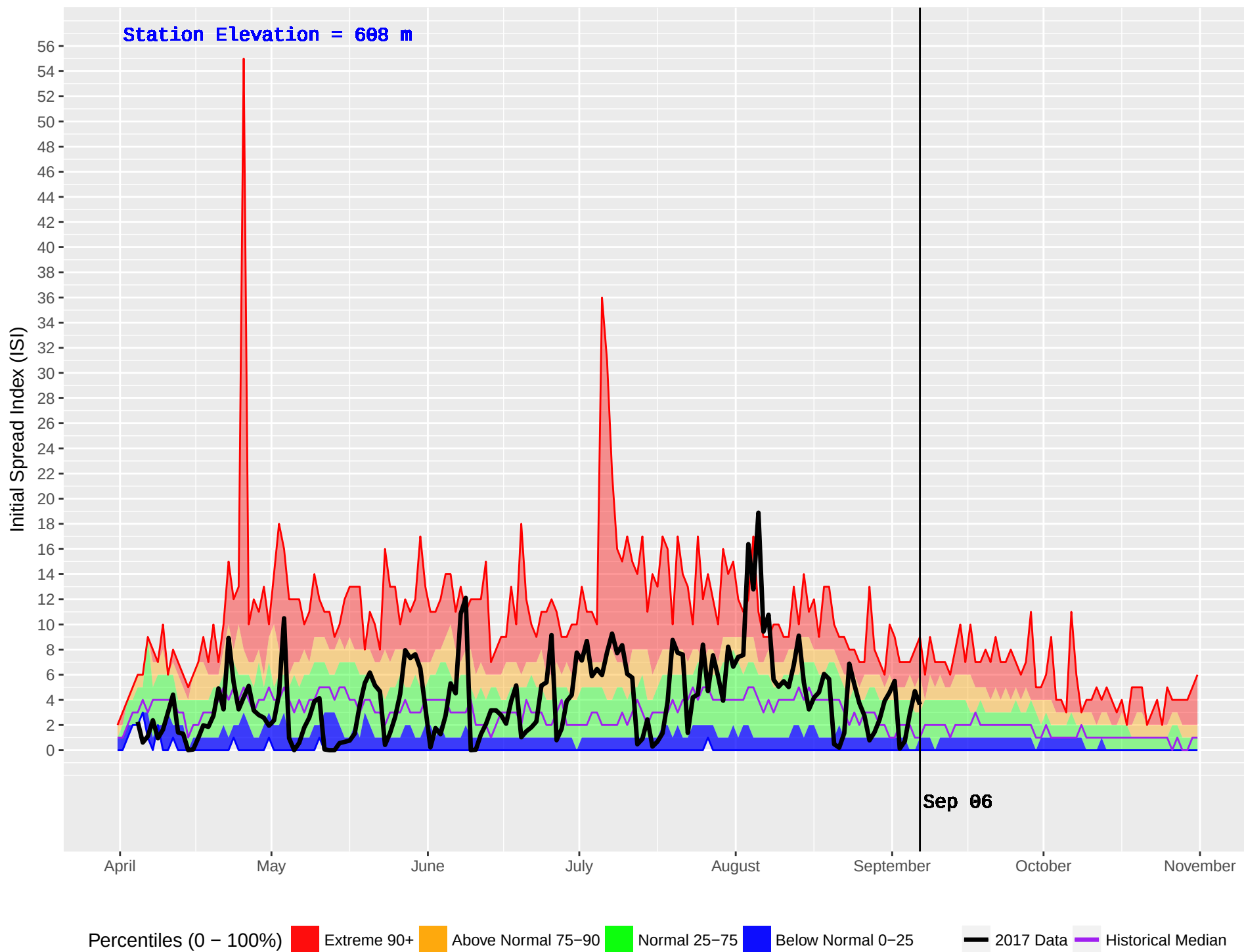
HOUSTON(DUNGATE) (162) : Historical (1974–2016) and Current (2017) Noon Initial Spread Index (ISI)
