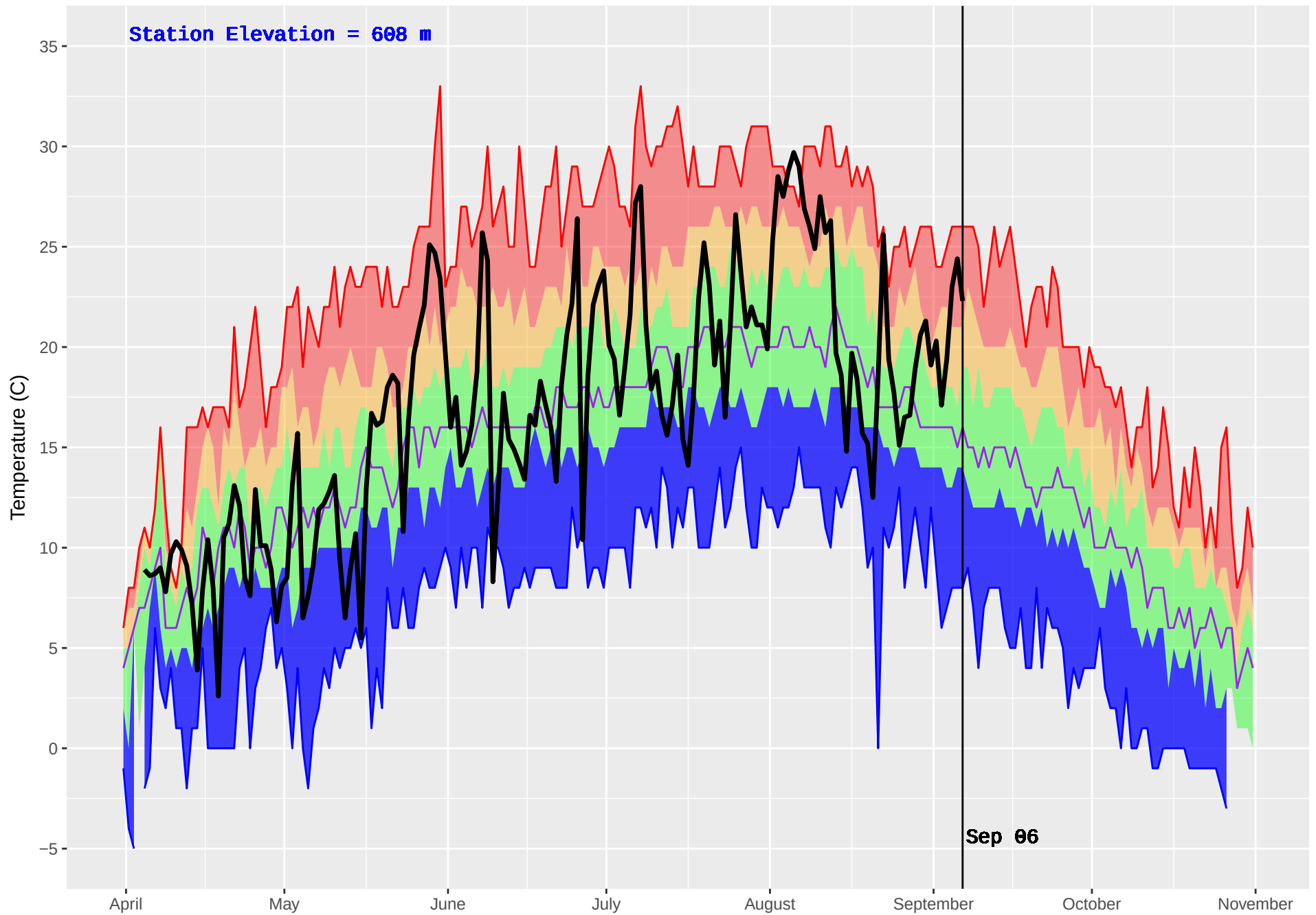
HOUSTON(DUNGATE) (162) : Historical (1974–2016) and Current (2017) Noon Temperature
