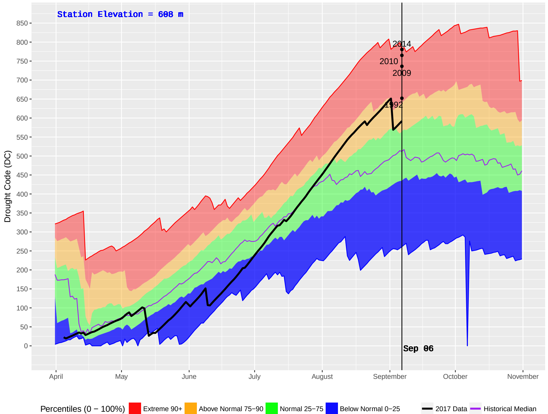
HOUSTON(DUNGATE) (162) : Historical (1974–2016) and Current (2017) Noon Drought Code (DC)
