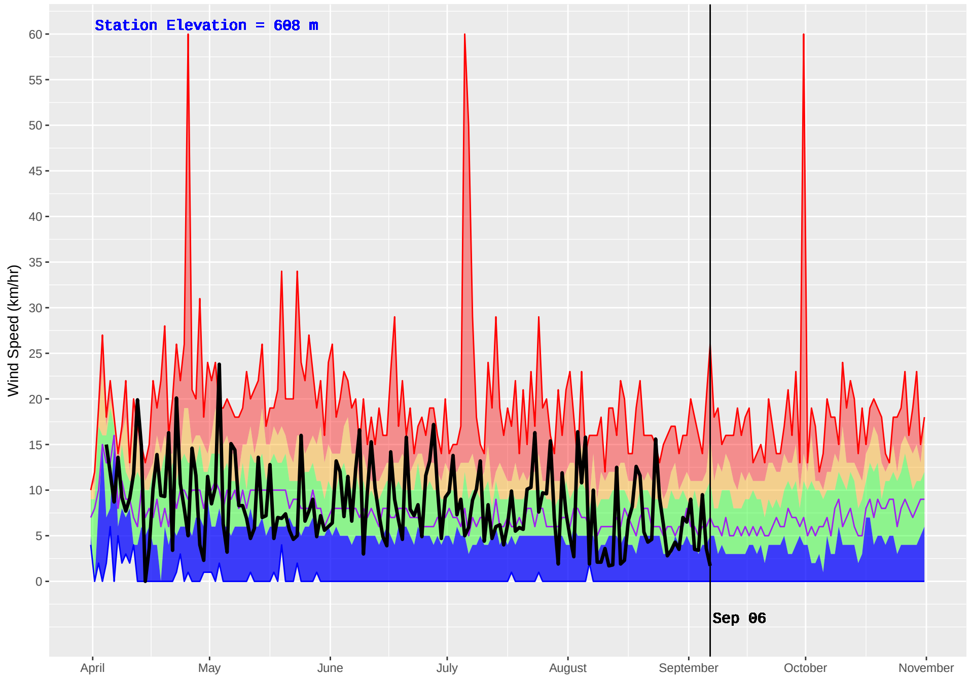
HOUSTON(DUNGATE) (162) : Historical (1974–2016) and Current (2017) Noon Wind Speed
